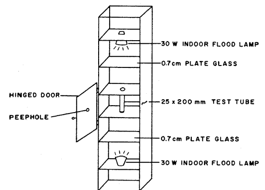
FIGURE 1. Black box for observing phototactic response of Daphnia in a test tube.
